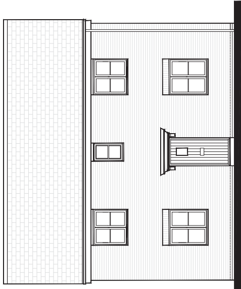
FRONT ELEVATION (C)
